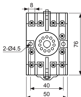
• 11-pin socket
