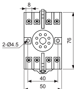
• 8-pin socket
